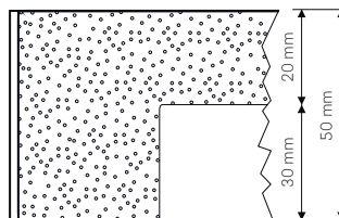
Chipboard core Anima in truciolare
